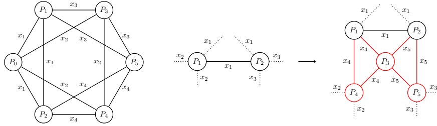
(a) Graph encoding of C_{base} , (b) Partial graph encoding of a clause before and after a non-red preserving transformation \mathcal{G}_{C_{base}}
